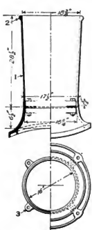
Figs. 466-467. Cast-Iron Taper Stack. American Loco. Co.
